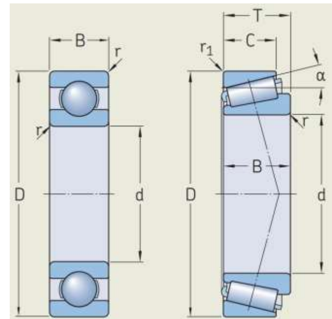
Fig. Boundary dimensions [SKF 2018]
