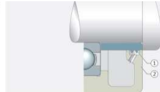
Splash rings
