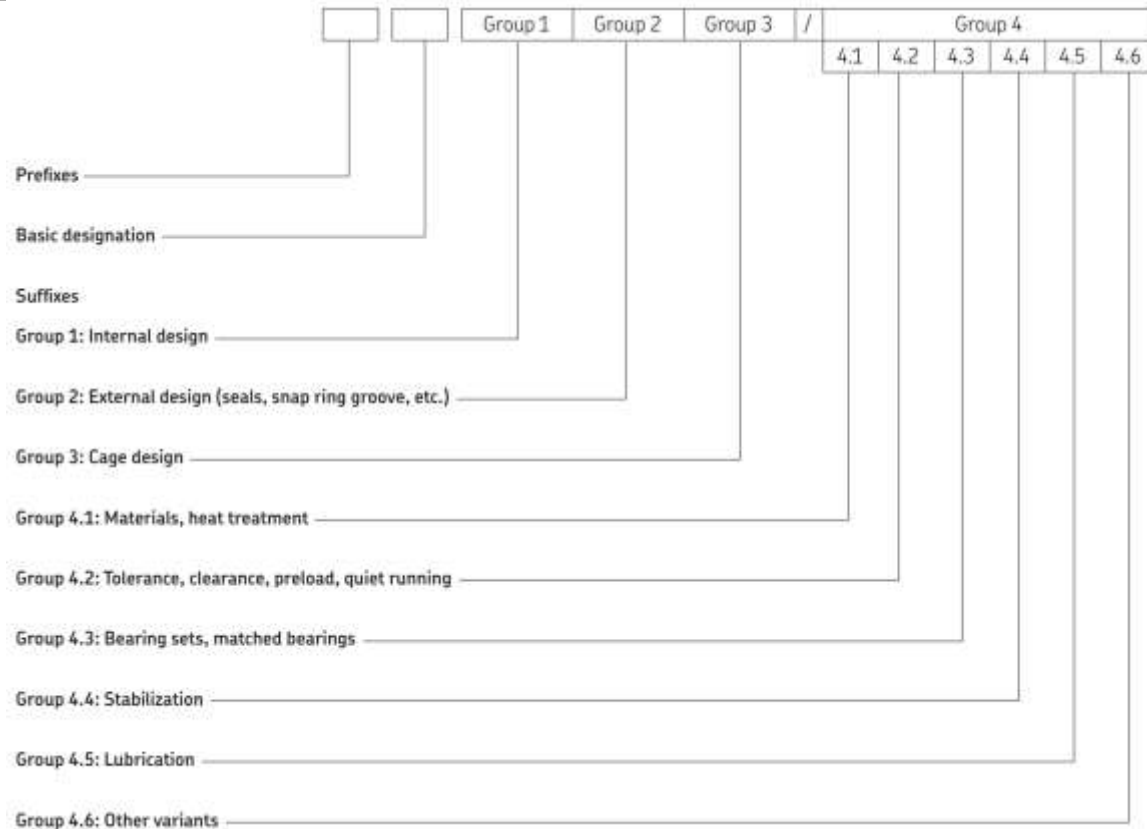
Fig. Detailed designation of a rolling bearing [SKF 2018]
